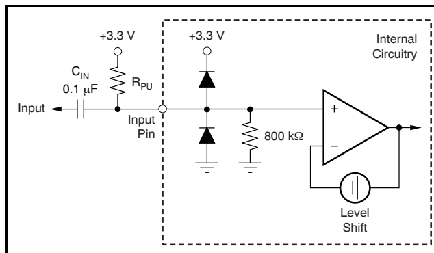
Figure 119. AC-Bias Input Mode Circuit Configuration
